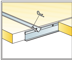
Connection between profiles with split pin
